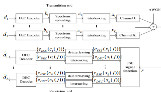
Figure 1. IDMA System [4].
