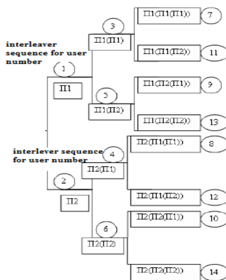
Figure 3. Masking of interleavers of TBI [6].
