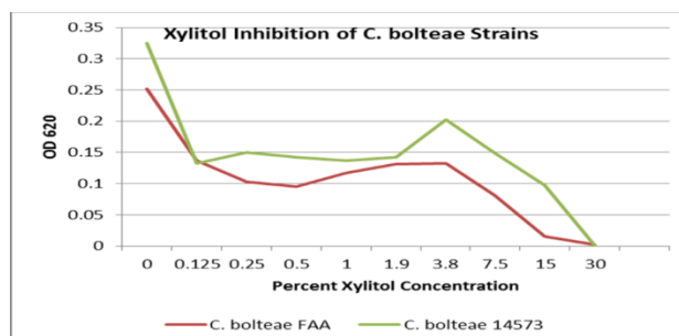
Figure 3. C. bolteae strains inhibited by a very low concentration of xylitol, but less so at a 2% level.
