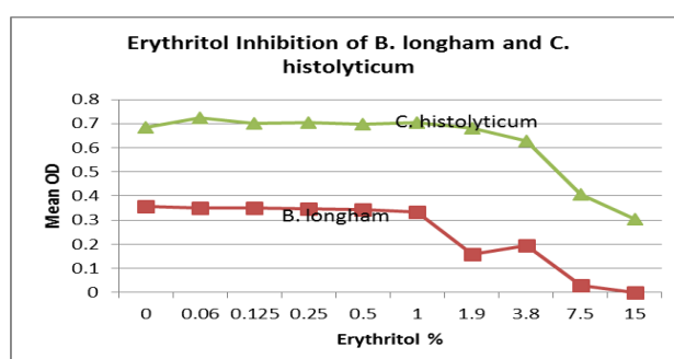
Figure 2. Erythritol inhibits at around a 2% concentration but inhibits the probiotic more than xylitol.
