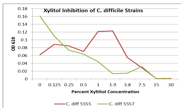
Figure 6. At 2% concentration, xylitol generally inhibit C. difficile strains, although C.diff5557 is inhibit in a more linear manner and at a lower concentration.
