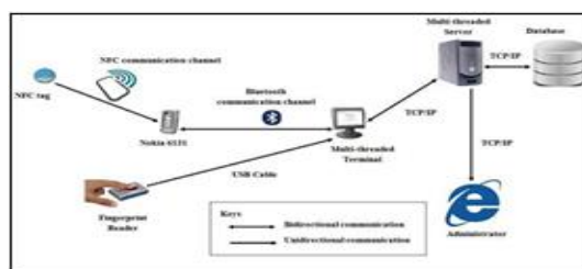
Figure 2. Bluetooth Based Attendance Management System [7] .
