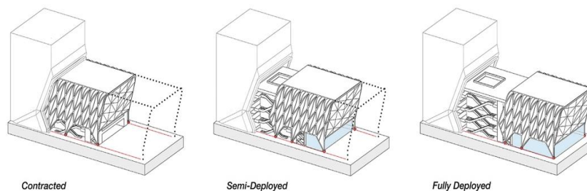
Figure 4. Deployment of the Envelope by moving cover [144].
