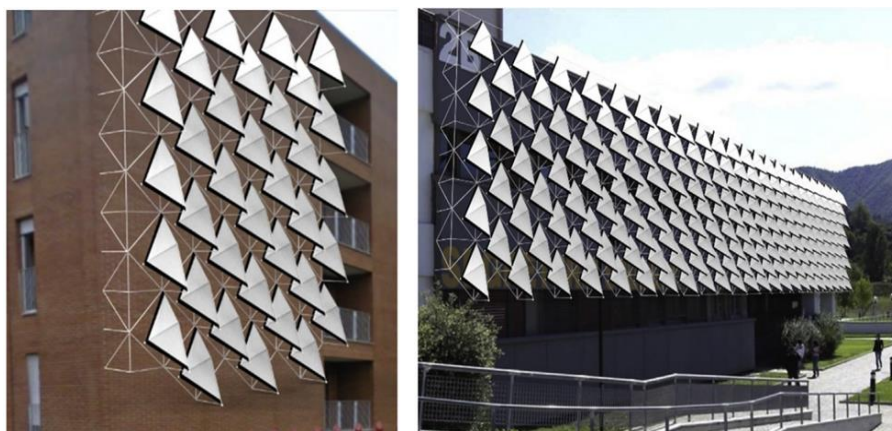
Figure 10. Blinking sail facades with fully opened configuration [101].
