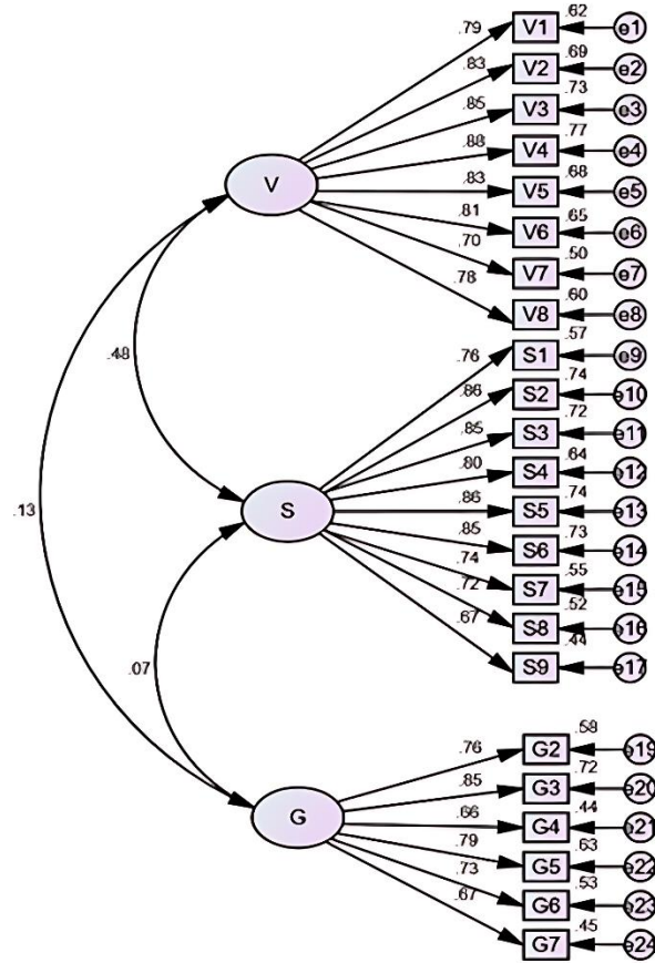
Figure 3. Model of First-Order Three-Factor Structure.
